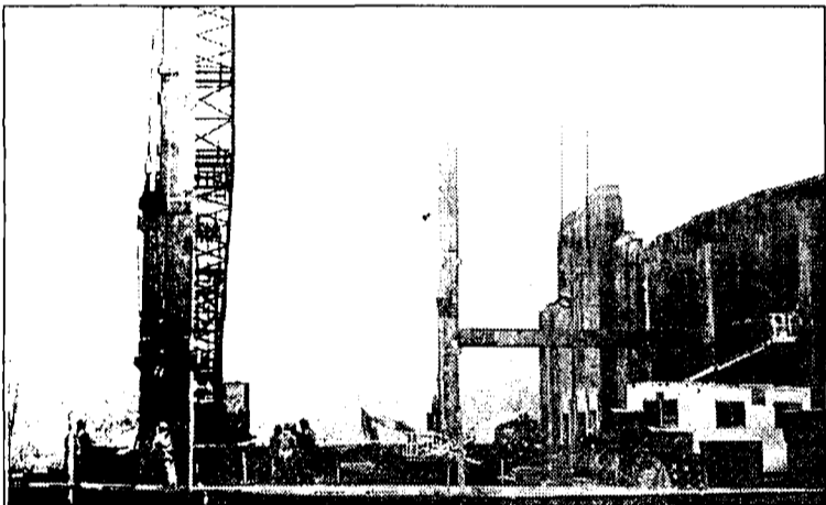
The Observer/Katie Kroemer The first of 276 concrete columns that will support the new and improved Notre Dame stadium was placed in the ground yesterday, the first major proof of progress.
